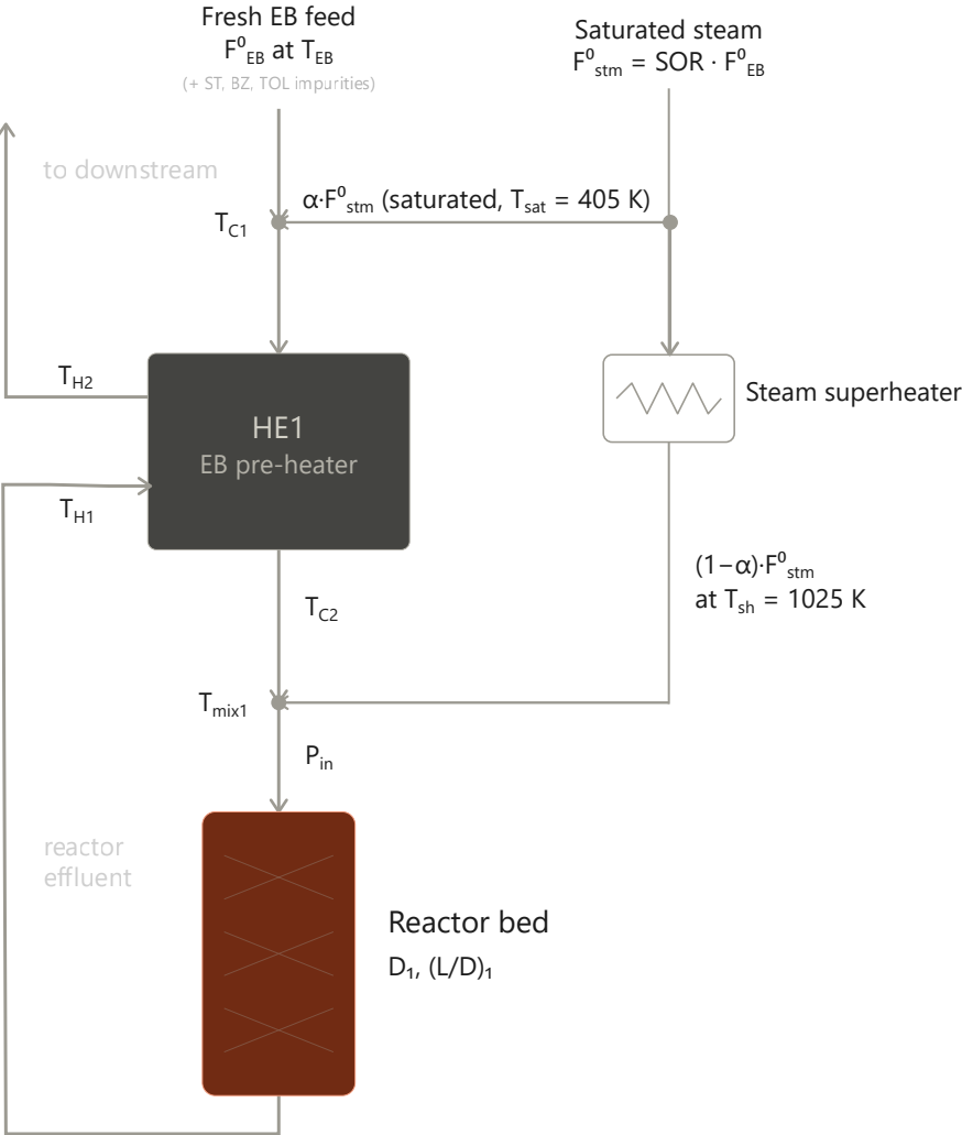
a. Single-bed (SB)
