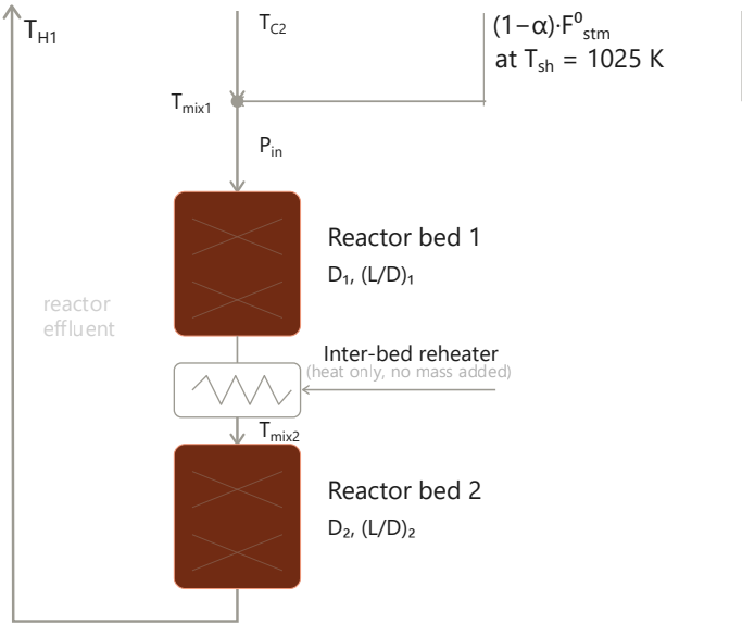
c. Double-bed (DB)
