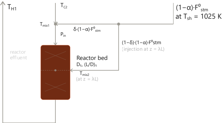
b. Steam-injected (SI)
